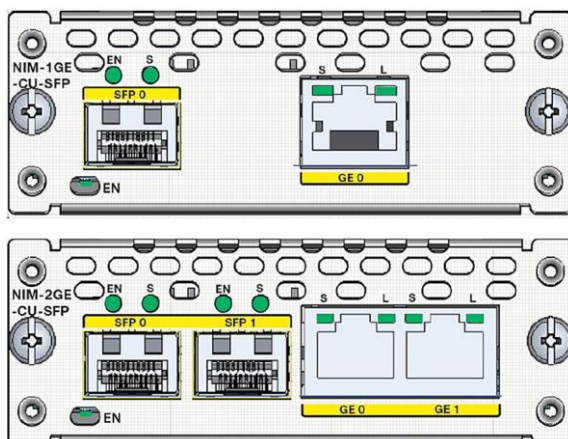
Figure 1. Cisco 1- and 2-Port Gigabit Ethernet WAN Network Interface Modules
